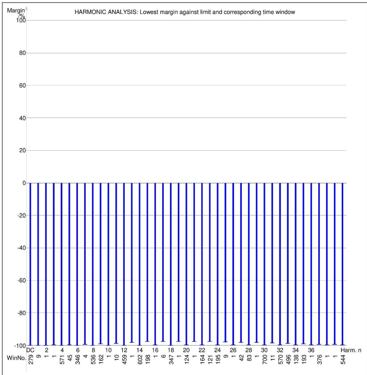
Graphical Harmonic Overview - EN61000-3-2 Class A
